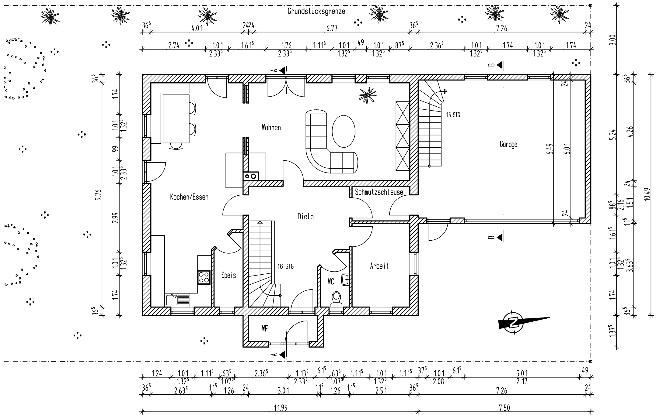
Grundriß Erdgeschoß
