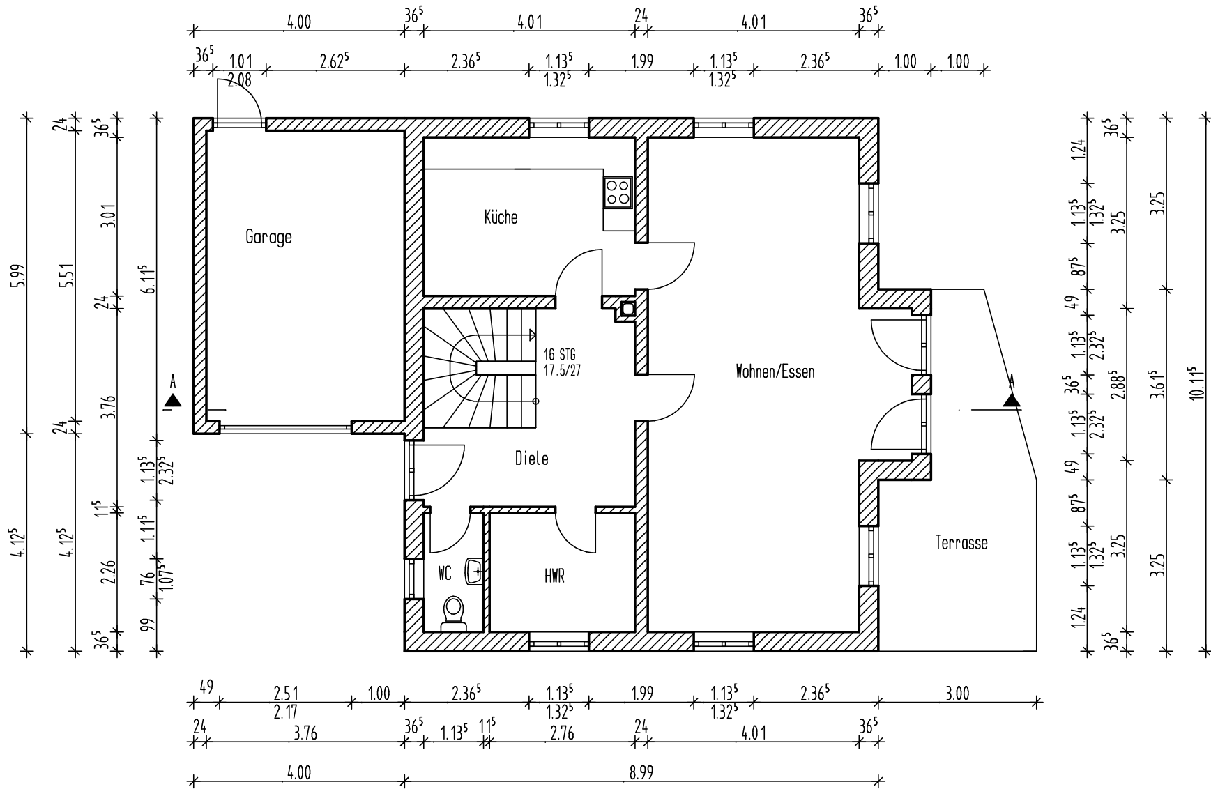
Grundriß Erdgeschoß
